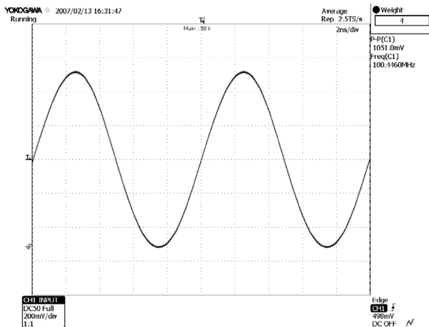
Large Signal Response output signal for 100 MHz, 200 \mu W modulated optical input signal (with 4 times averaging)
