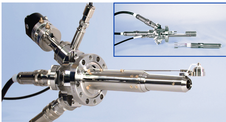
EFG-7 Electron Gun with Deflection (Inset shows gun demounted)
